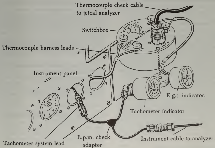
FIGURE 10-72. Switchbox and r.p.m. check adapter connections.
